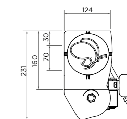
Loggia Pose Face
