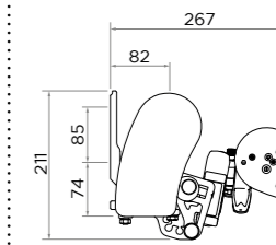
Perle Volant Pose Face
